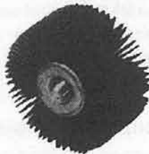
Coated Abrasive Flap Wheels Aluminum Oxide — 2-1/2" Diameter x 1" Wide. Includes 1/4"-20 Male Mandrel • 90830 60 Grit • 90831 80 Grit
